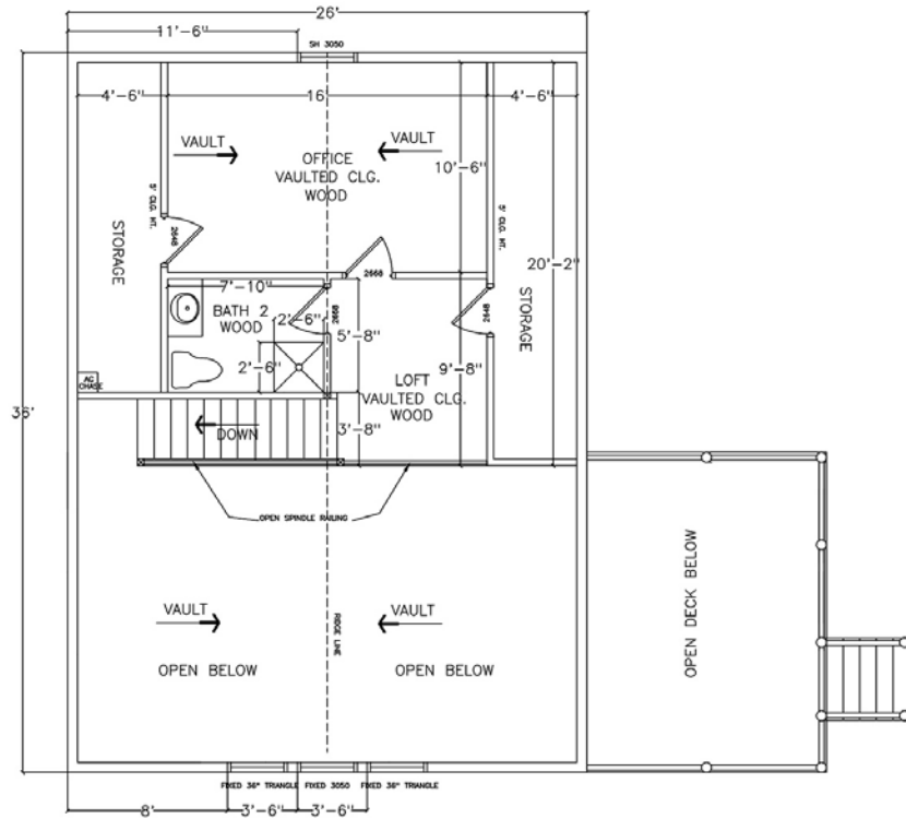
2ND LEVEL FLOOR PLAN
