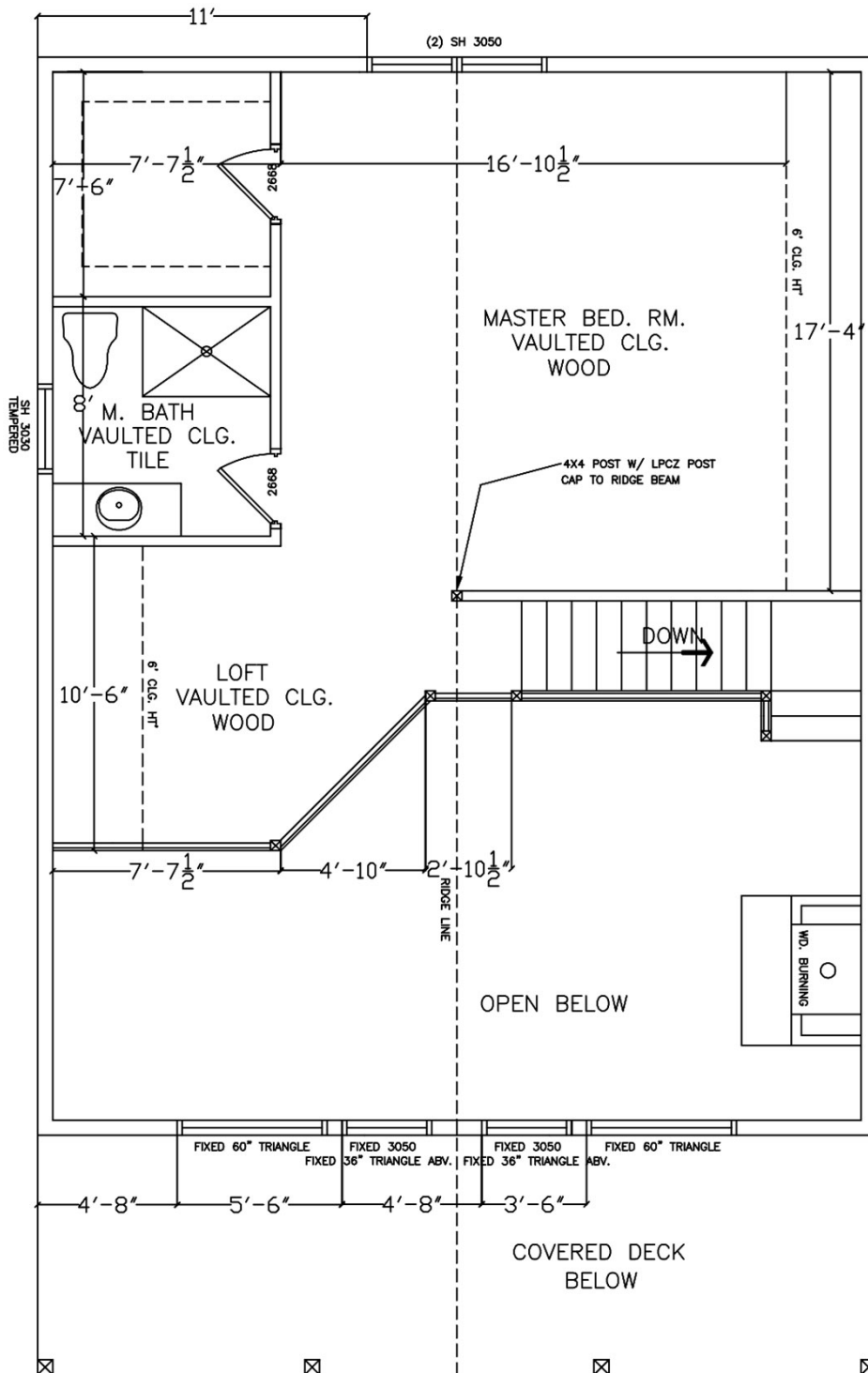
2ND LEVEL FLOOR PLAN
