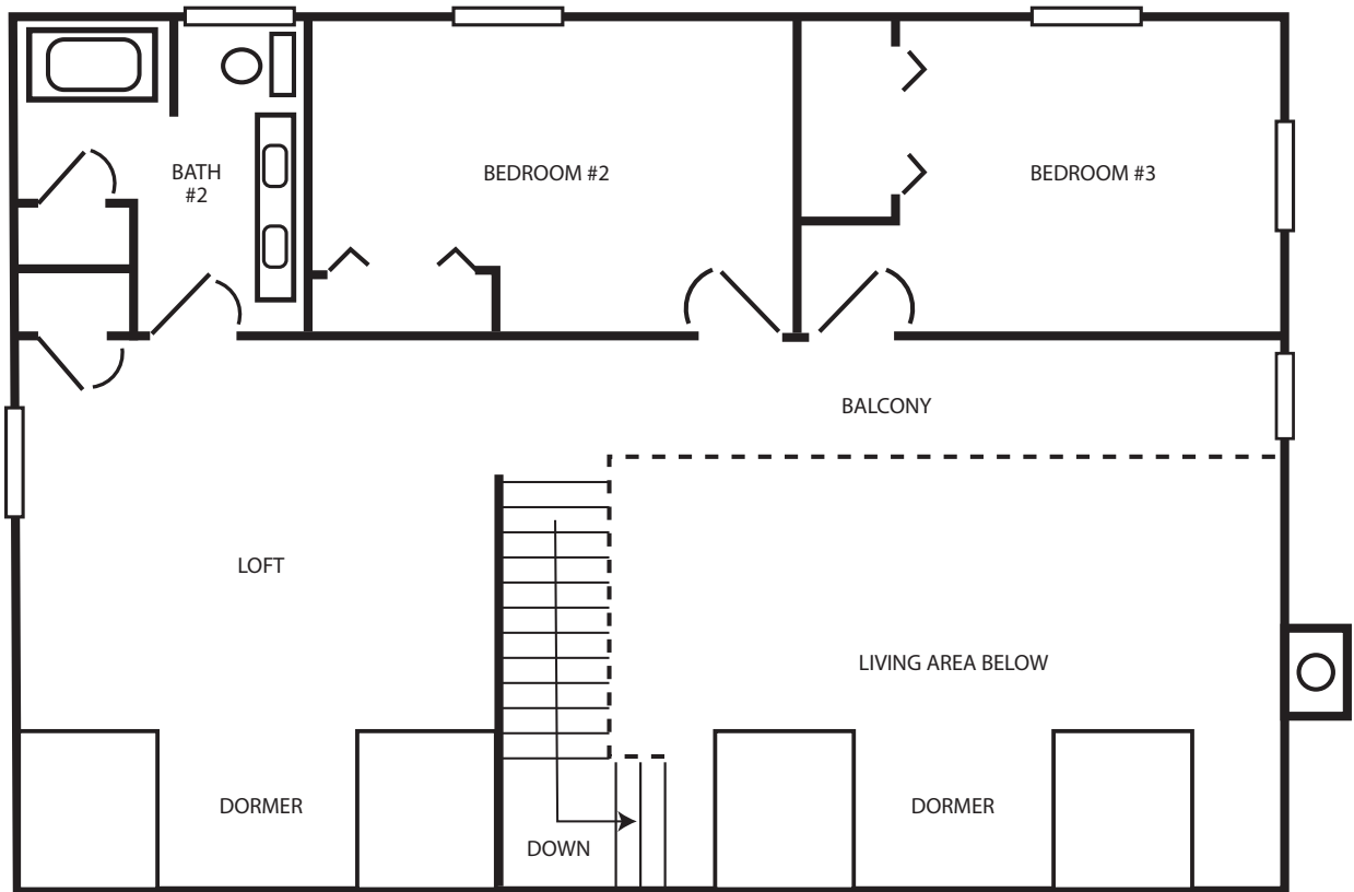
2ND LEVEL FLOOR PLAN
