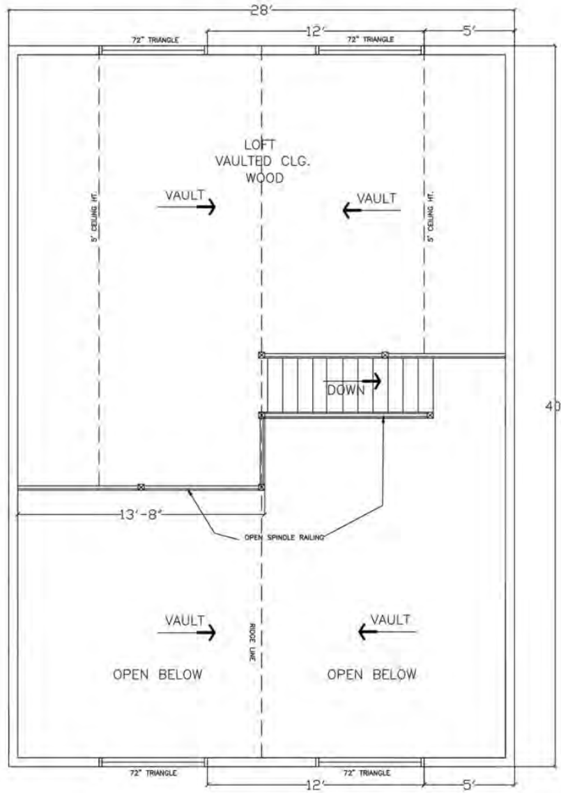
2ND LEVEL FLOOR PLAN
