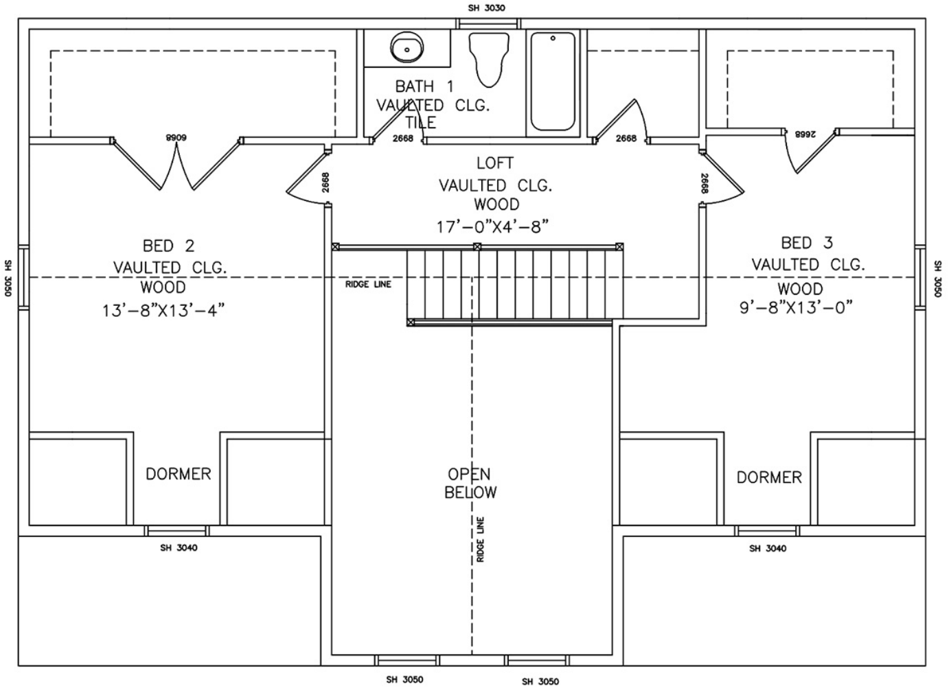
2ND LEVEL FLOOR PLAN
